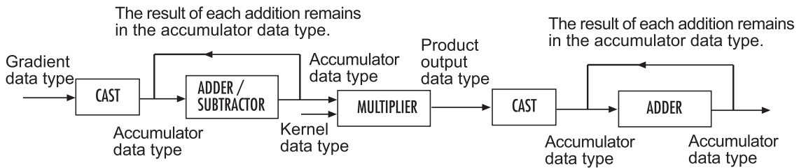
Data type diagram for product algorithm
